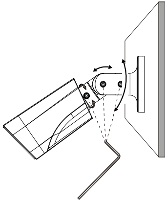
Figure 3-3 Adjusting the monitoring direction
