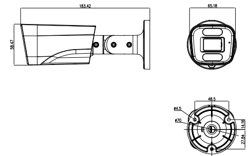
Figure 2-3 Zoom lens Dimensions (Unit: mm)
