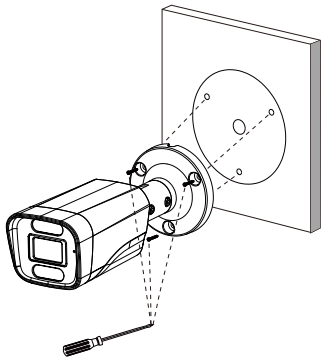
Figure 3-2 Installing camera
